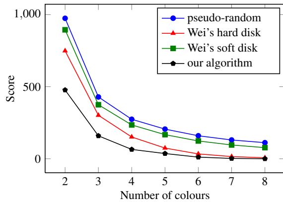
Figure 5: Results using the score described by Equation 8.
